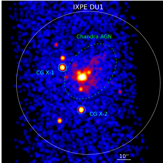
Figure 1. Chandra image of the Circinus galaxy ( 2' \times 2' ). The green dashed ellipse marks the Chandra extraction region for the AGN (see Sect. 2.2 for the details). The cyan dotted lines encircle the ULXs CG X-1 and CG X-2. The white dotted circle corresponds to the IXPE DU1 extraction region.
