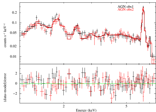
Figure 8. Chandra /ACIS spectra of the AGN with the best-fitting model in the 1–8 keV band. The black and red coloured crosses correspond to observation 1 and 2, respectively.
