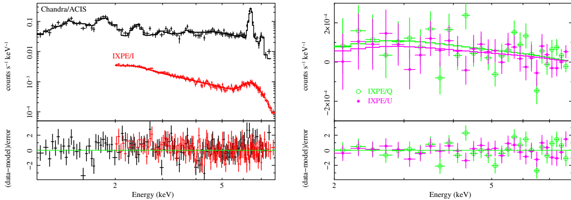
Figure 3. Left panel: Chandra/ACIS and IXPE I (flux) spectra of the Circinus galaxy with the best-fitting model and the residuals. Right panel: IXPE Q and U Stokes spectra with the best-fitting model and the residuals. Note the different scale from the left panel. In both panels, IXPE spectra are grouped for plotting purposes only (with SETPLOT GROUP in xSPEC ).
