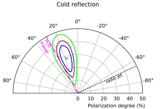
Figure 5. Contour plot of the polarization degree and angle for the cold reflector. The blue, red and green lines correspond to the 68, 90 and 99 per cent confidence levels, respectively. The black dashed line marks the direction of the radio jet, while the magenta dash-dotted line marks the direction of the inner \text{H}_2\text{O} maser disc.
