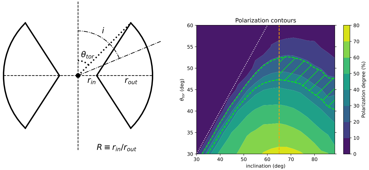
Figure 6. Left panel: Sketch of the torus geometry assumed for polarimetric modelling. The torus opening angle \theta_{\text{tor}} and the observer inclination i are both measured from the symmetry axis. Right panel: Contour plots of the constant polarization degree calculated for scattering off a torus, on the \theta_{\text{tor}} - i plane. The white dotted line corresponds to the equality \theta_{\text{tor}} = i ; the condition for the obscuration of the central source is \theta_{\text{tor}} < i . The green dashed curves enclose the 68 per cent confidence level region on the measured polarization for the cold reflector in the Circinus galaxy. The orange dashed line marks the inclination of the host galaxy, likely a lower limit to the torus inclination (as discussed in the text). The green hatches mark the region of the parameter space consistent with all the observational constraints.
