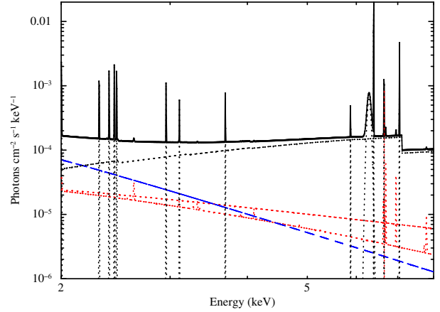
Figure 4. Best-fitting total model (black solid line) in the 2–8 keV band, together with the contribution of various components: cold reflection (black dotted line), warm reflection (blue dashed line), ULXs (red dotted lines).
