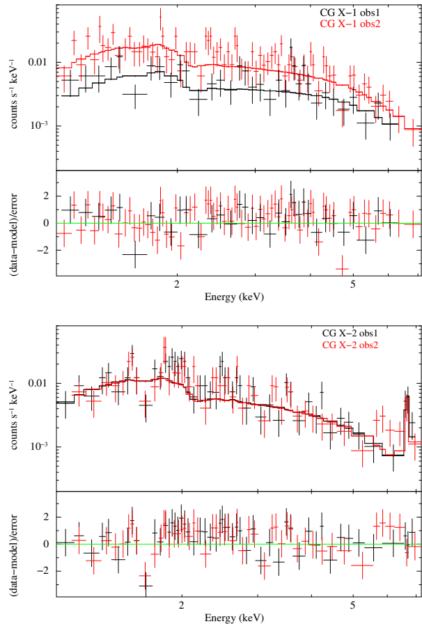
Figure 7. Chandra /ACIS spectra of CG X-1 (top) and CG X-2 (bottom) with the best-fitting model in the 1–8 keV band. The black and red coloured crosses correspond to observation 1 and 2, respectively.
