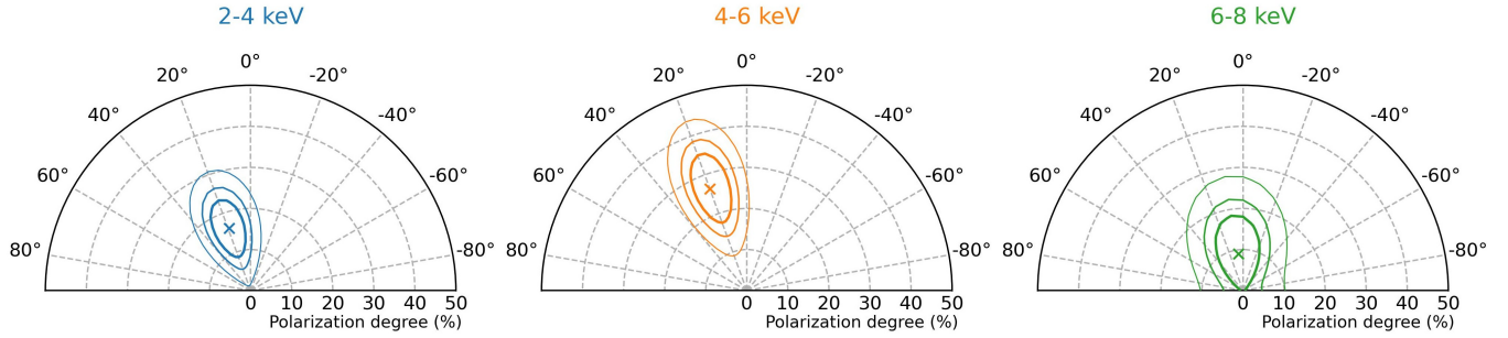
Figure 2. Contour plots of the polarization degree and angle, measured with xSPEC , at the 68, 90 and 99 per cent confidence levels, in the 2–4 (left panel, light blue), 4–6 (middle panel, orange) and 6–8 keV (right panel, green) energy bands.
